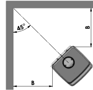
3410 corner installation
