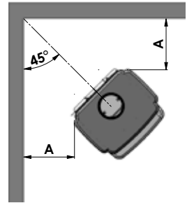
3440 corner installation
